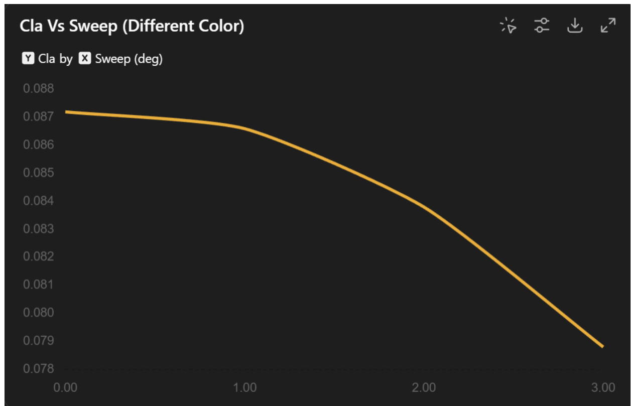
Cla graph for sweep variation
