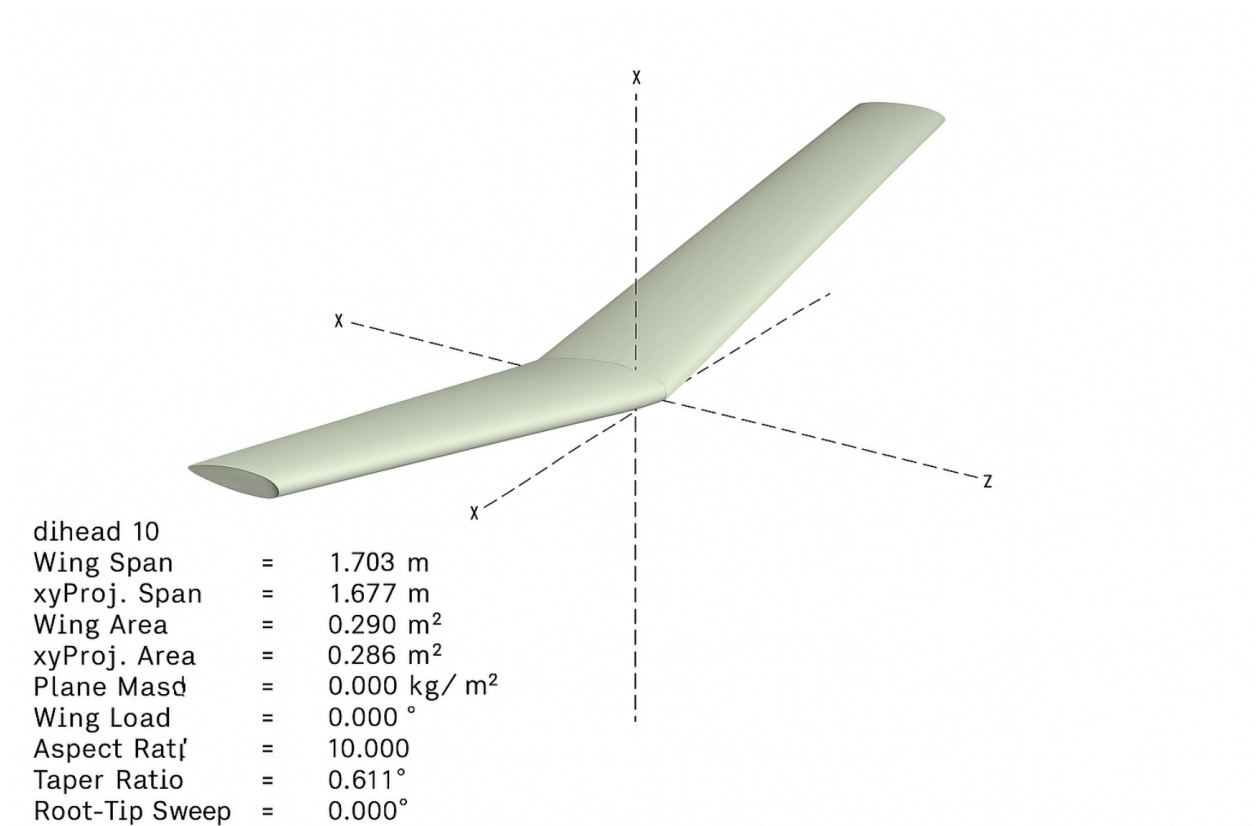
10 Degree dihedral angle wing NACA 0024^
