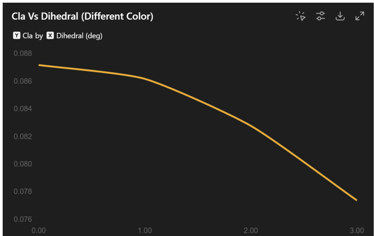
Cla graph for dihedral angle variation
